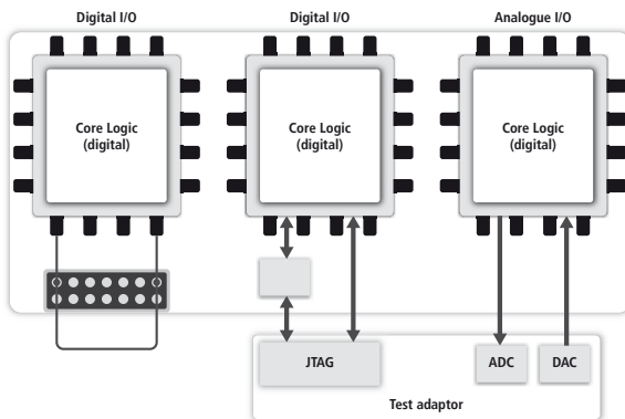
Figure 25: Including peripheral connectors in connectivity tests
