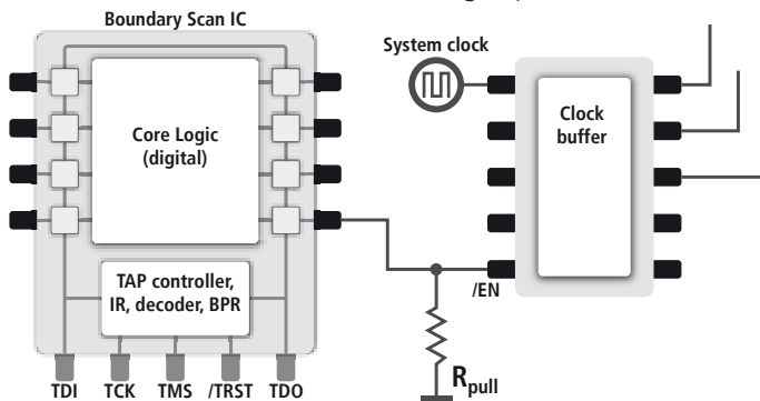
Figure 14: Example for clock control
