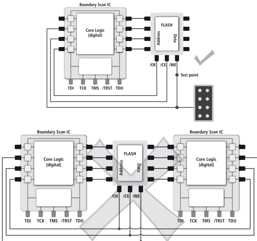
Figure 17: Flash memory access from a single Boundary Scan IC
