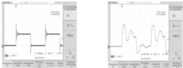
Figure 6: Considerable overshoots due to signal reflections
