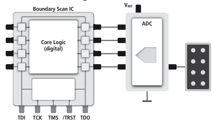
Figure 21: ADC test
