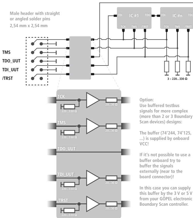
Figure 8: Example design of a complete scan chain including termination
