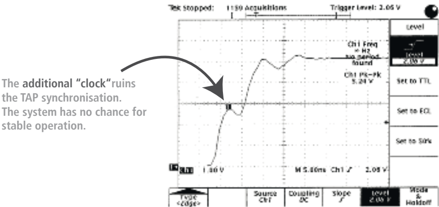
Figure 9: „Extra Clock“ at the rising edge due to inappropriate termination
