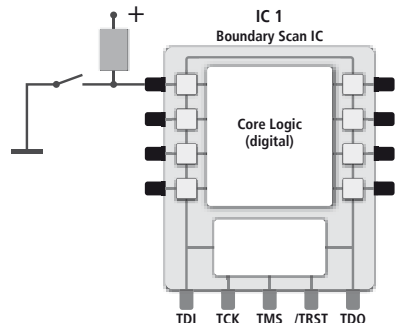
Figure 23: Switch test
