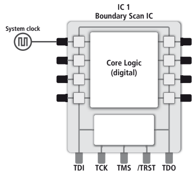
Figure 24: Clock signals
