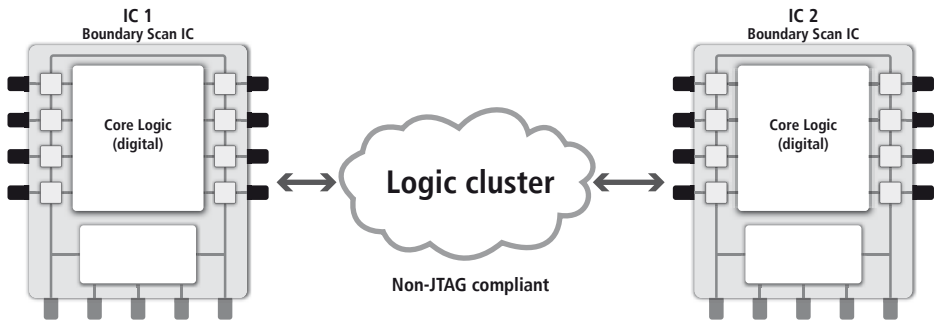
Figure 15: Logic cluster surrounded by Boundary Scan ICs
