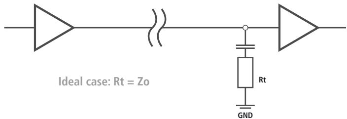
Figure 7: Termination with pull-down resistor and capacitor
