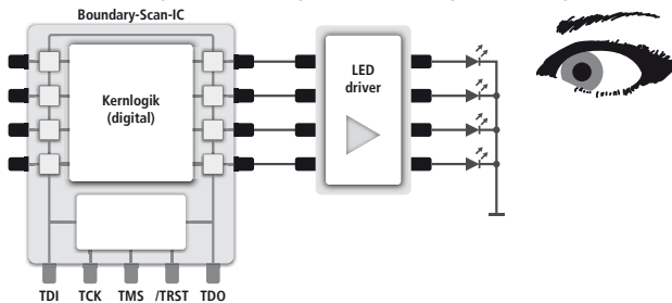
Figure 22: LED test
