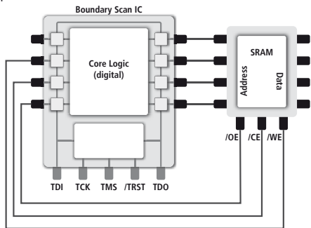
Figure 16: Memory and Boundary Scan ICs
