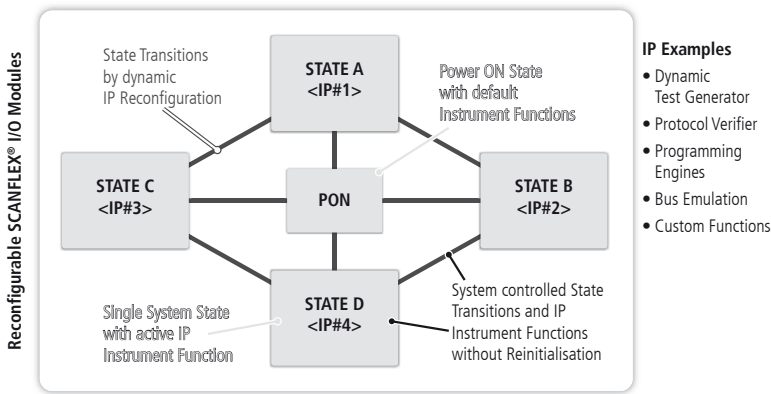
Figure 26: Reconfigurable VarioCore® I/O Module
