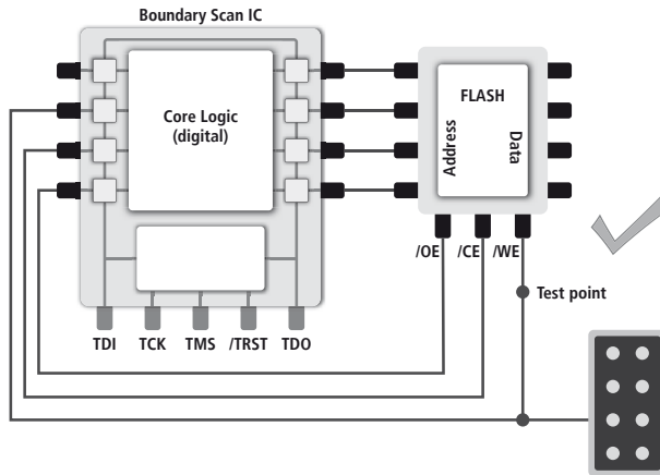
Figure 18: External control of /WE Signals
