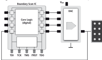
Figure 20: DAC test
