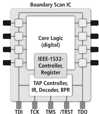
Figure 2: IEEE 1532 device
