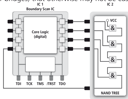
Figure 19: NAND-Tree test
